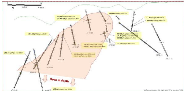
Long section (10m envelope for representation of drill hole traces) including drill intercept highlights (AgEq) and projection of the mineralized shoot
